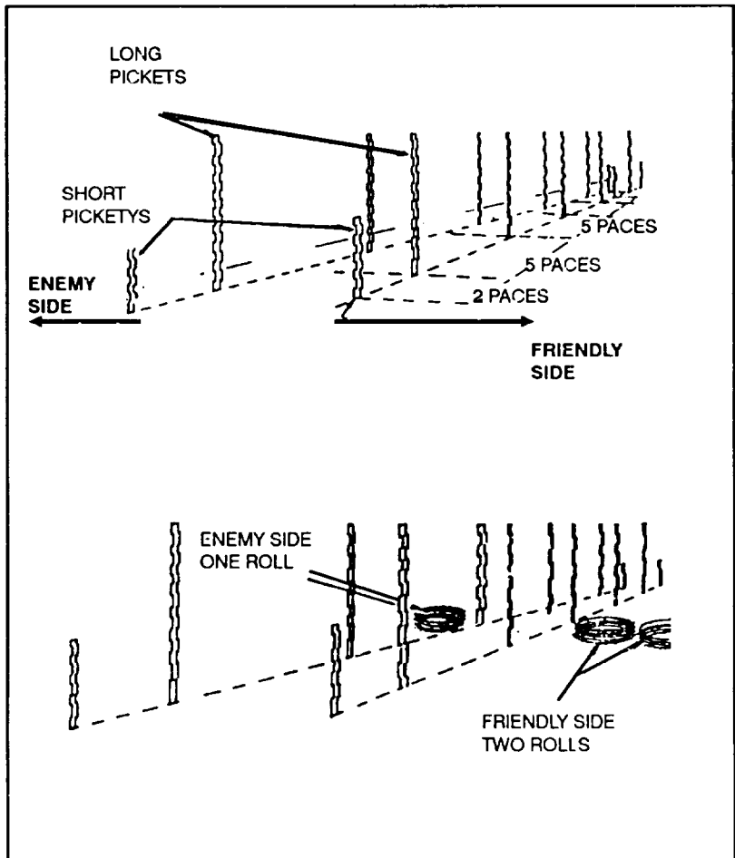
Figure 2-76. Concertina fence.
